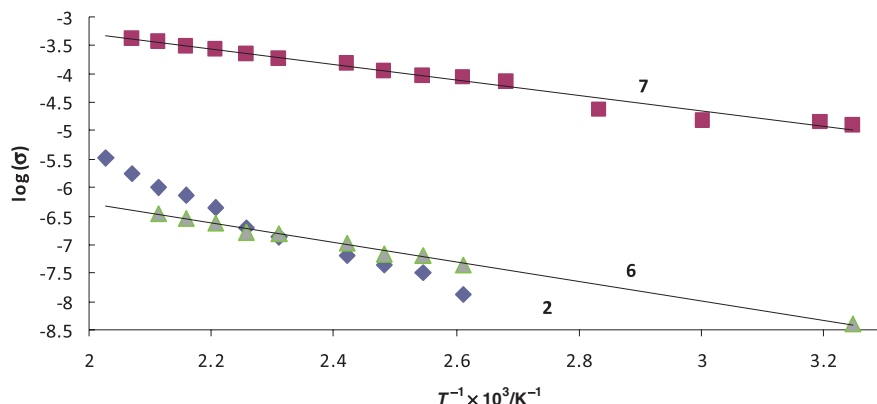
Figure 7. Temperature dependence of electrical conductivities of the complexes: rectangular bar 2 , cubic bar 6 , triangular bar 7 .
