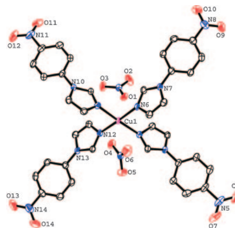
Figure 3. ORTEP view of 7 at 30% probability of thermal ellipsoids (H atoms excluded for clarity). Selected bond lengths and angles: Cu(1)–N(9) = 1.994(3) \text{\AA} , Cu(1)–N(3) = 2.007(3) \text{\AA} , Cu(1)–N(12) = 2.015(3) \text{\AA} , Cu(1)–N(6) = 2.019(3) \text{\AA} , N(9)–Cu(1)–N(3) = 177.45(12)°, N(9)–Cu(1)–N(12) = 86.46(11)°, N(3)–Cu(1)–N(12) = 95.68(11)°, N(9)–Cu(1)–N(6) = 92.43(11)°, N(3)–Cu(1)–N(6) = 85.38(11)°, N(12)–Cu(1)–N(6) = 177.17(11)°.
